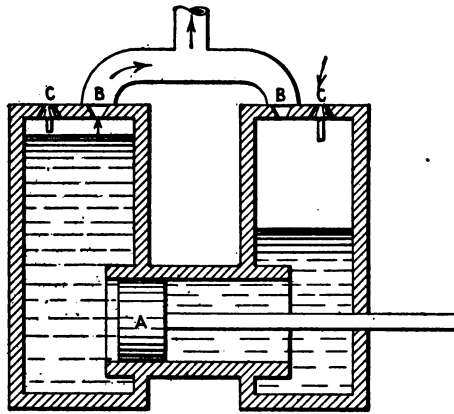
FIG. 40.—Hydraulic piston compressor.
